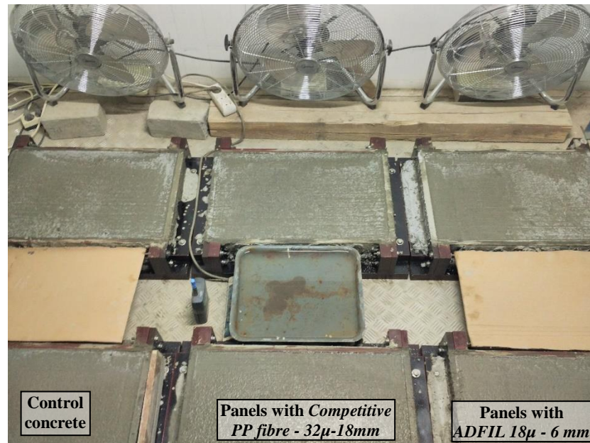
Fig. 2. Specimens (from left to right): two control panels, two panels made of concrete with Competitive PP fibre - 32µ-18mm fibers, and two panels made of concrete with ADFIL 18µ - 6 mm fibers
